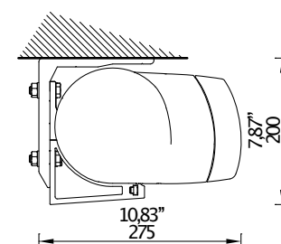
Ceiling installation
