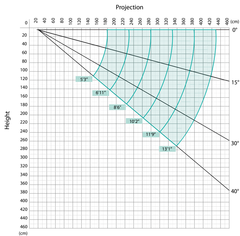
Covering diagram - Wall/ceiling installation
