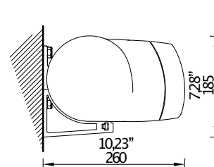
Wall installation
