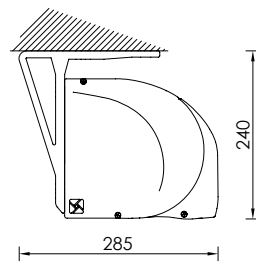
Ceiling installation
