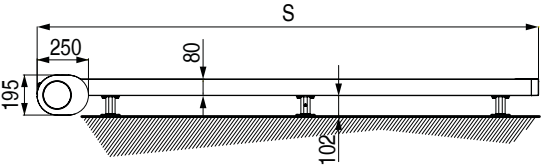
General technical plan (mm)
