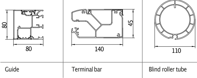
Profiles dimensions (mm)
