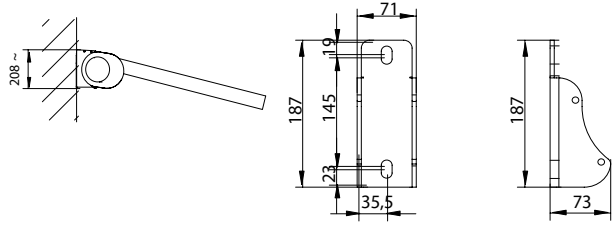
Wall fixing (mm)
