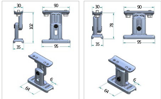
Ground connections (mm)
