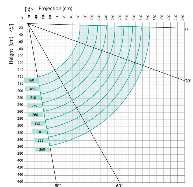
Wall installation 80°
