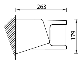
Wall installation
