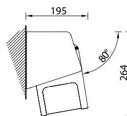
Wall installation 80°
